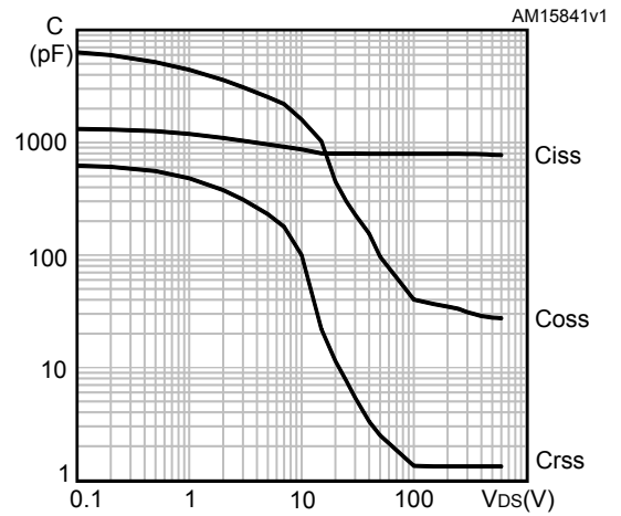
Figure 8. Capacitance variations
