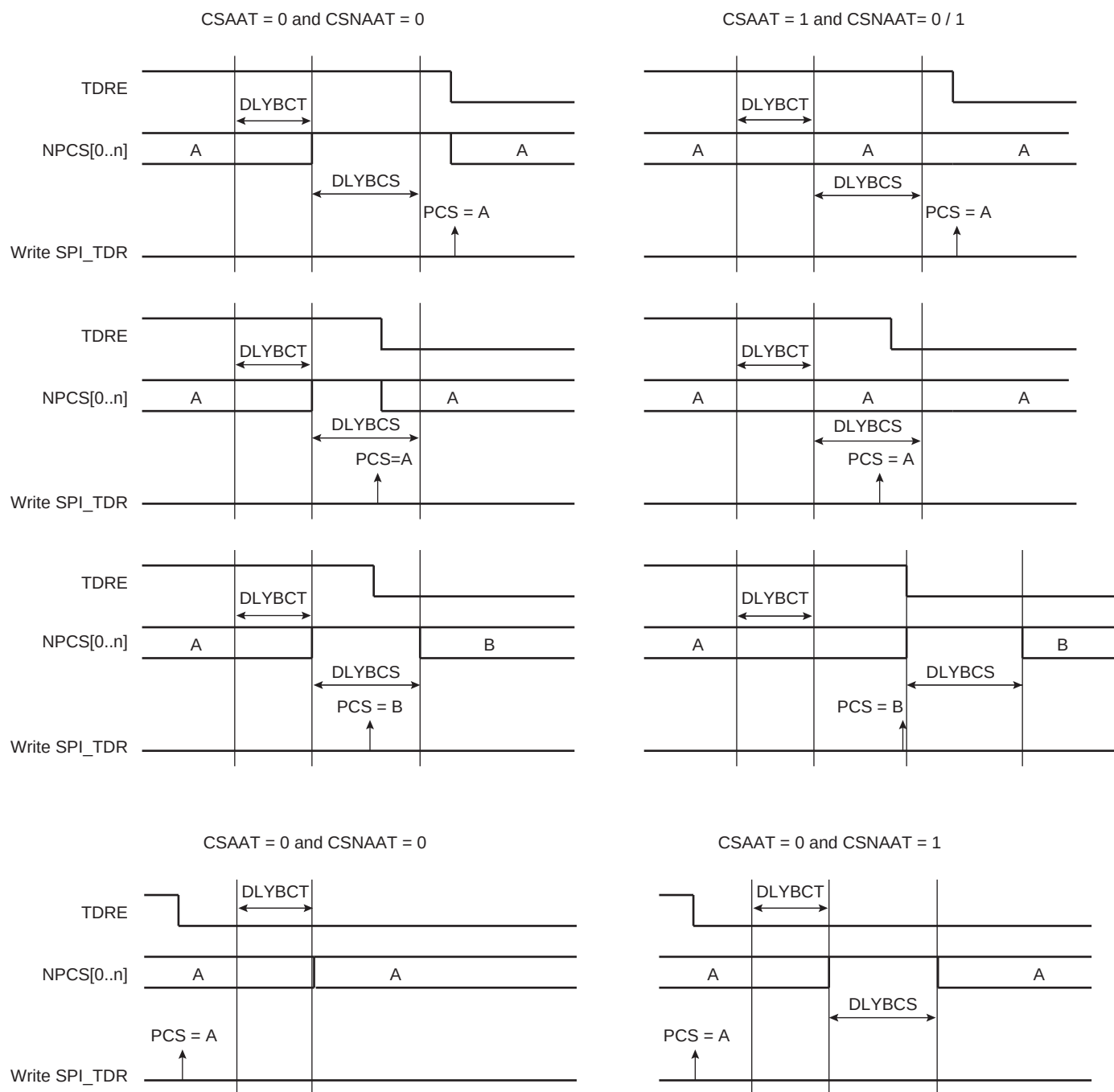
Figure 33-11. Peripheral Deselection
