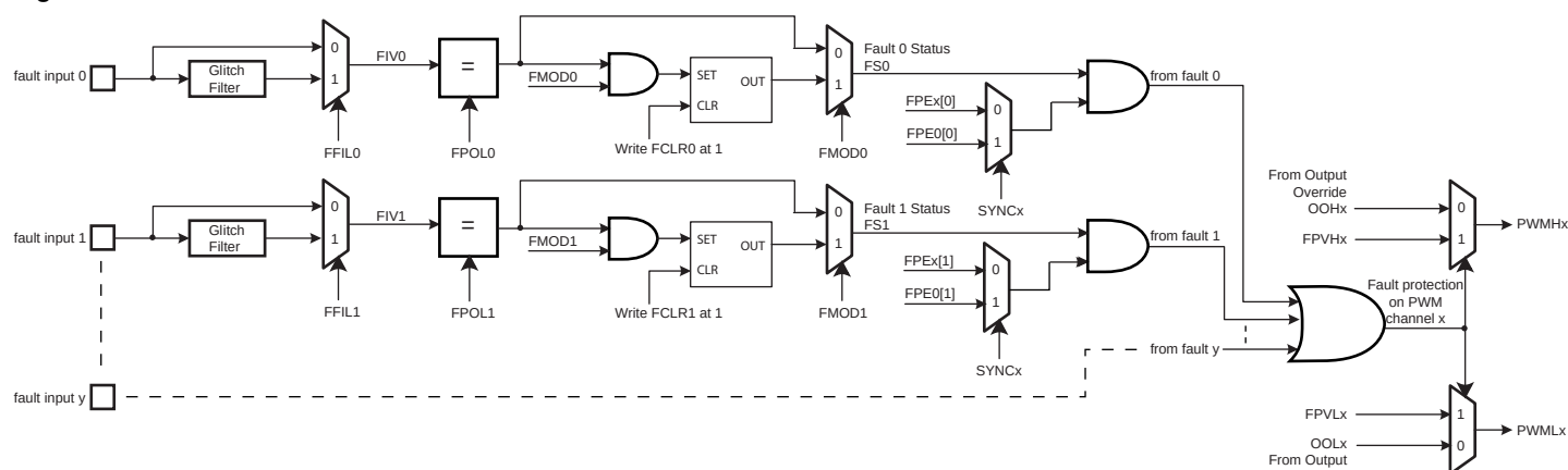
Figure 39-9. Fault Protection
