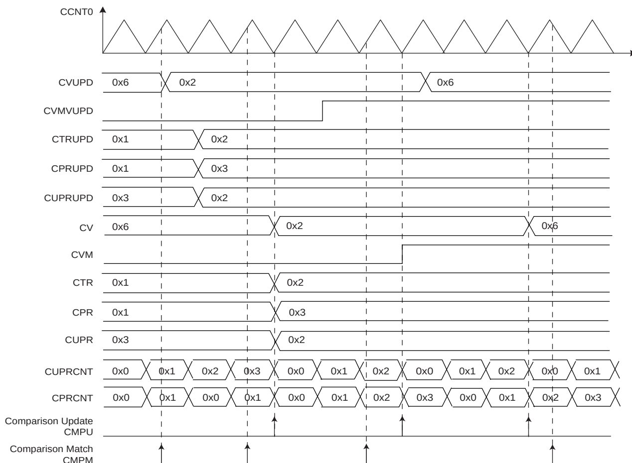
Figure 39-15. Comparison Waveform
