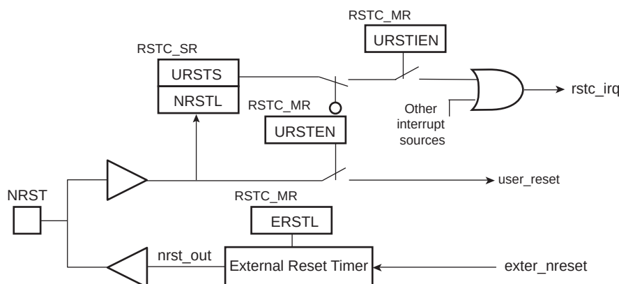
Figure 14-2. NRST Manager
