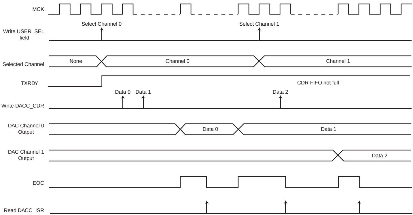
Figure 43-2. Conversion Sequence
