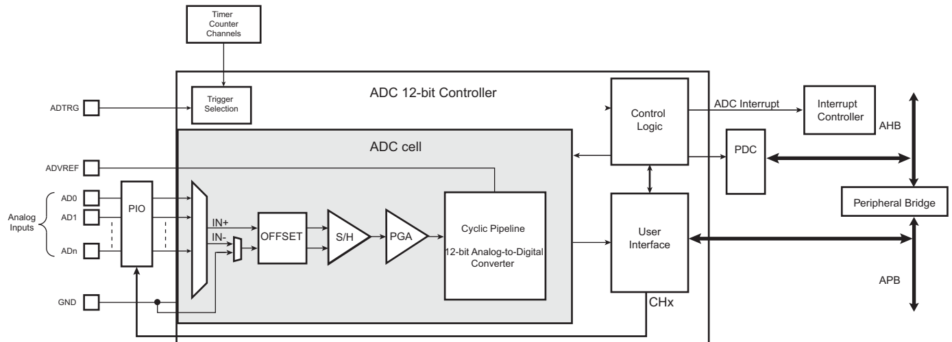
Figure 42-1. Analog-to-Digital Converter Block Diagram
