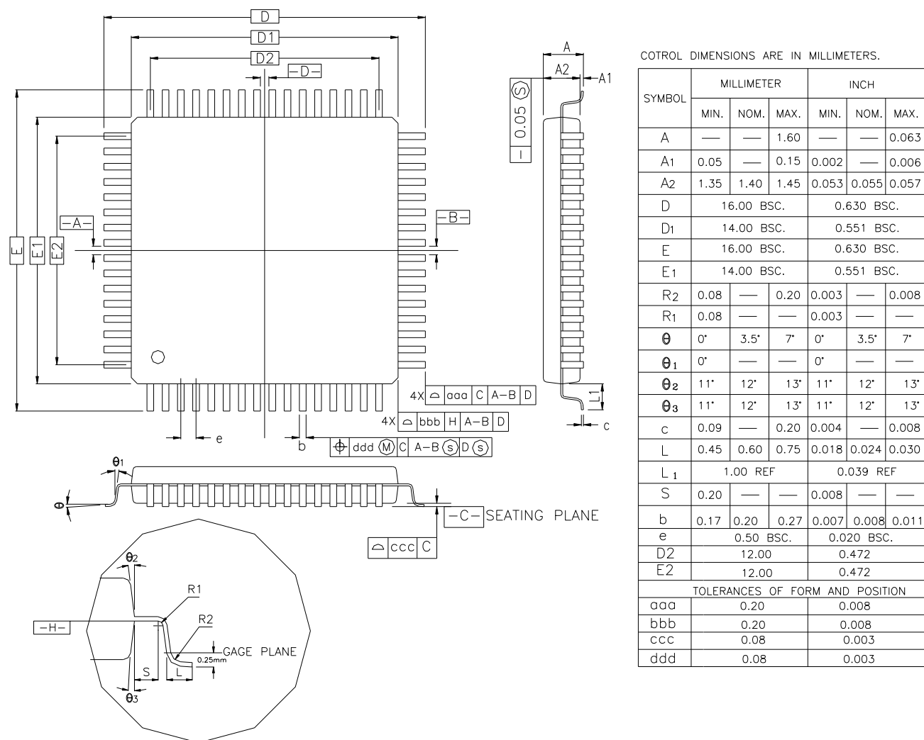
Figure 45-1. 100-lead LQFP Package Mechanical Drawing
