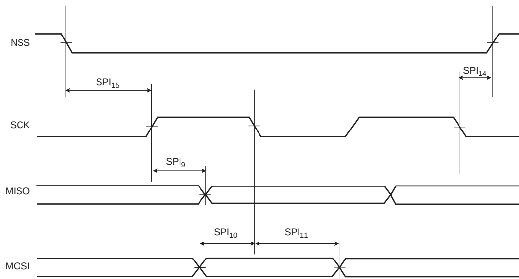
Figure 44-39. USART SPI Slave Mode: (Mode 0 or 3)
