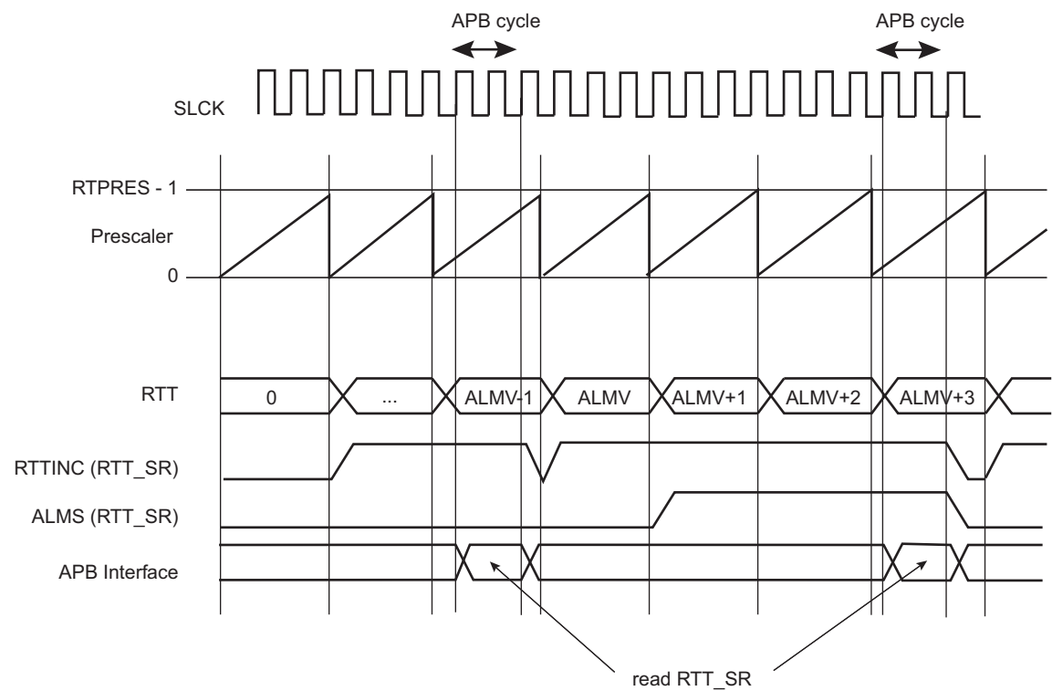
Figure 15-2. RTT Counting
