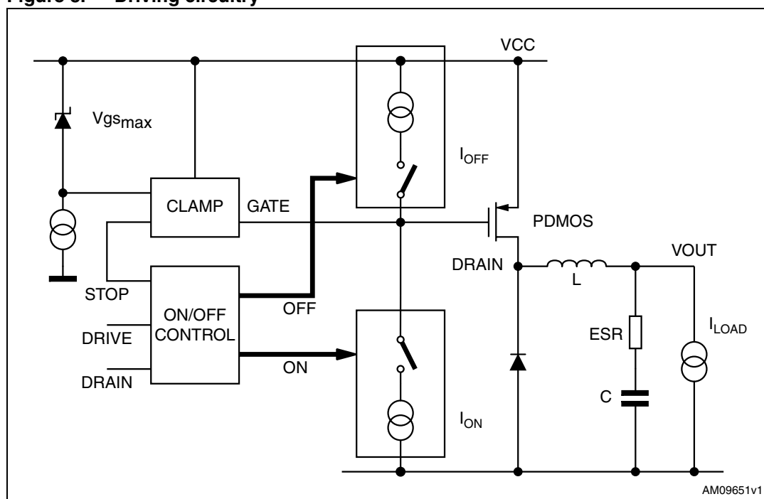
Figure 8. Driving circuitry
