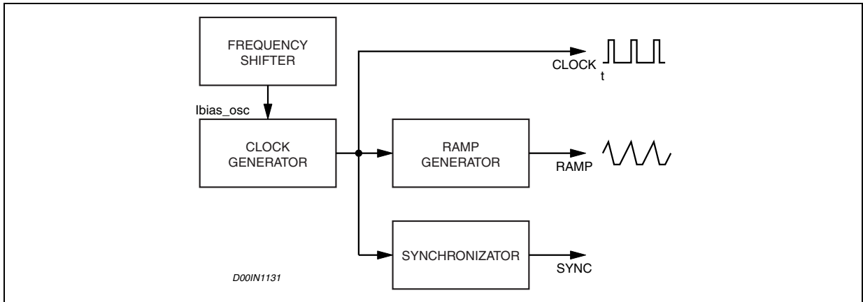
Figure 6. Oscillator Circuit
