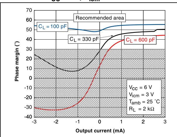
Figure 25. Phase margin vs. output current, at V_{CC} = 6\text{ V} , V_{icm} = 3\text{ V} and T = 25\text{ }^{\circ}\text{C}
