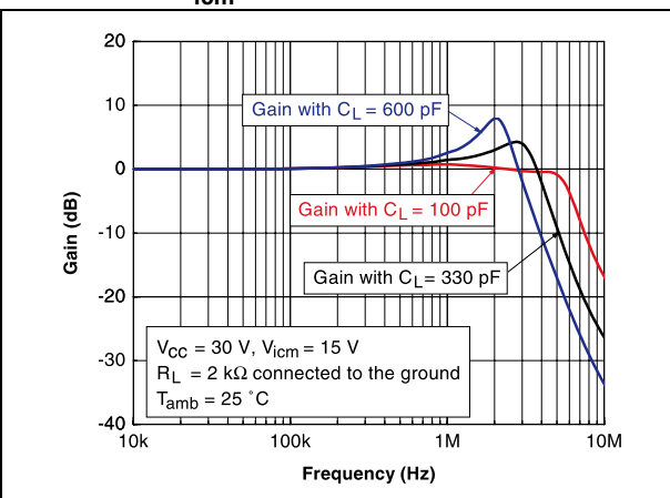
Figure 21. Frequency response for different capacitive load at V_{CC} = 30\text{ V} , V_{icm} = 15\text{ V} and T = 25\text{ }^{\circ}\text{C}
