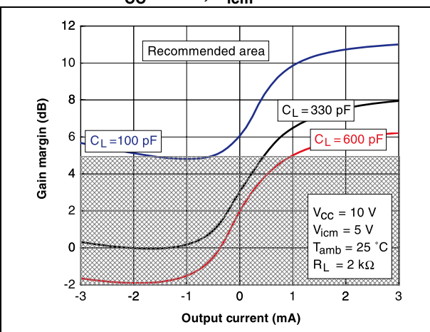
Figure 23. Gain margin vs. output current, at V_{CC} = 10\text{ V} , V_{icm} = 5\text{ V} and T = 25\text{ }^{\circ}\text{C}
