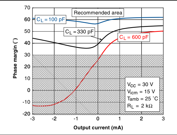
Figure 27. Phase margin vs. output current, at V_{CC} = 30\text{ V} , V_{icm} = 15\text{ V} and T = 25\text{ }^{\circ}\text{C}
