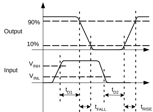
Figure 7. Inverting Timing Diagram
