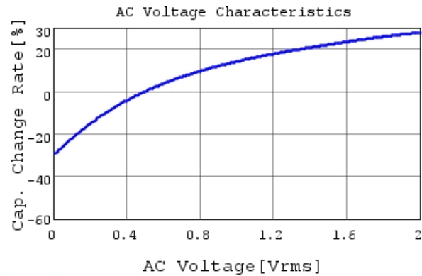
GRM32ER71C226MEA8 C-AC Voltage capchange, Dc
