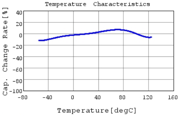
GRM32ER71C226MEA8 C-Temp. capchange, DC0.0V,
