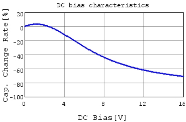
GRM32ER71C226MEA8 C-DC bias capchange, 25.0c
