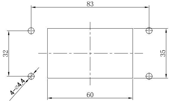
Panel cut out for use without Hoods/housings
