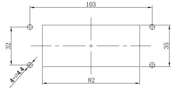
Panel cut out for use without Hoods/housings
