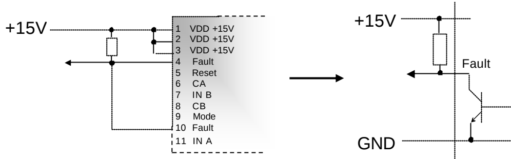
Figure 3.4 Fault output
