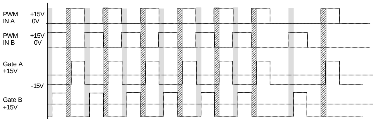
Figure 3.2 Switching diagram with interlock delay times
