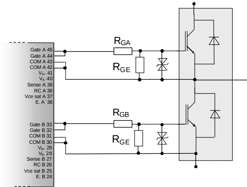
Figure 3.61 Gate connection
