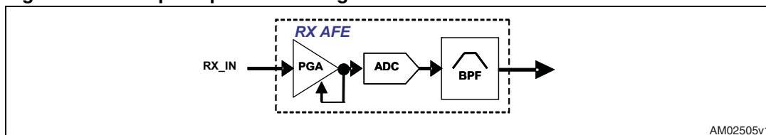
Figure 6. Reception path block diagram
