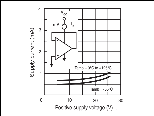
Figure 6. Supply current
