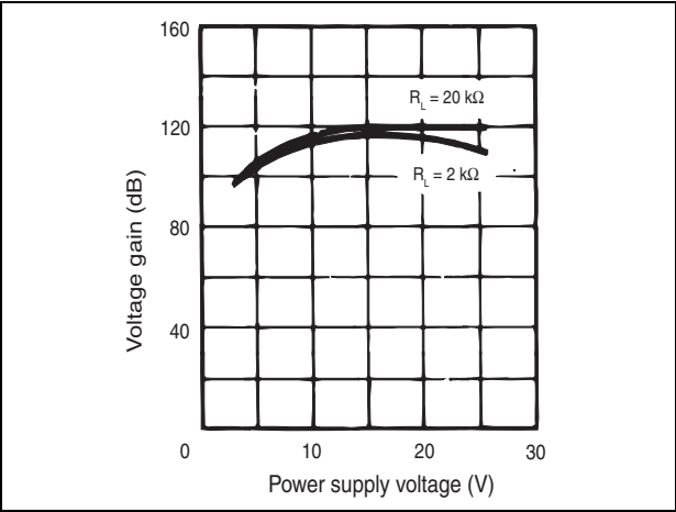
Figure 18. Voltage gain
