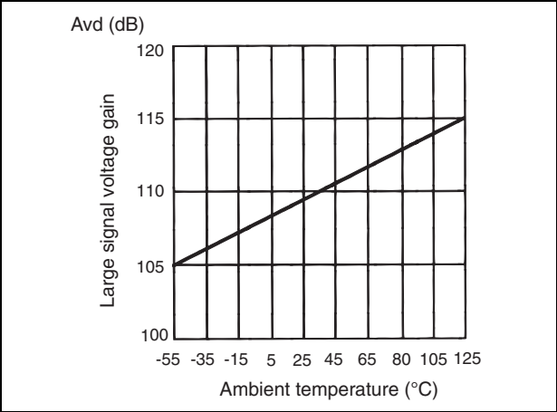
Figure 18. Voltage gain
