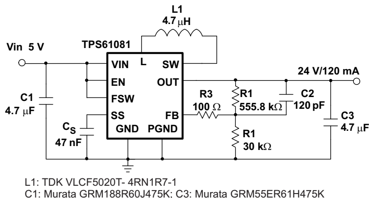
Figure 22. 5 V to 24 V, 120 mA Step-Up DC-DC Converter
