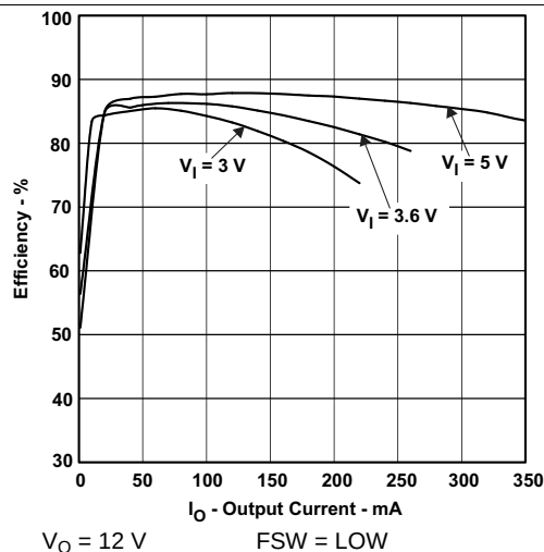
Figure 4. TPS61081 Efficiency
