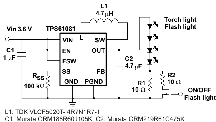
Figure 21. 50 mA Torch Light and 100 mA Flash Light
