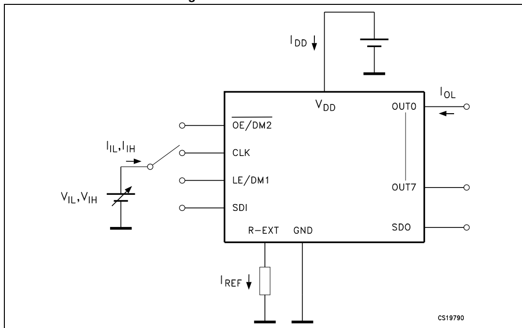
Figure 15. DC characteristics
