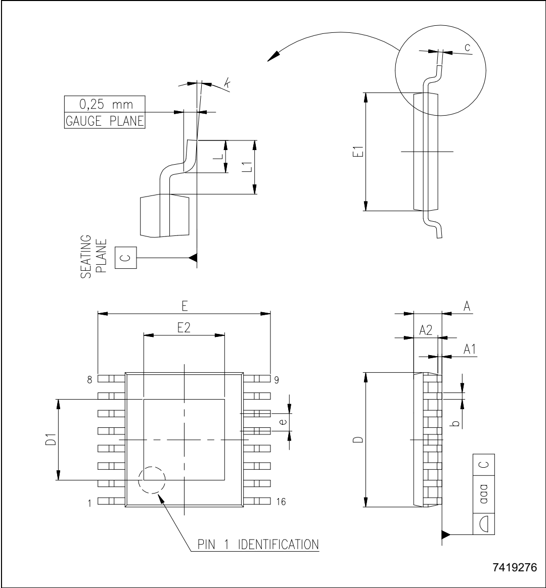
Figure 19. HTSSOP16 exposed pad drawing
