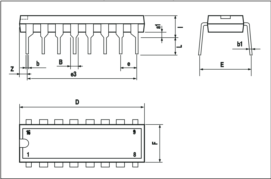
Figure 18. DIP16 drawing
