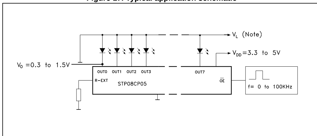
Figure 17. Typical application schematic
