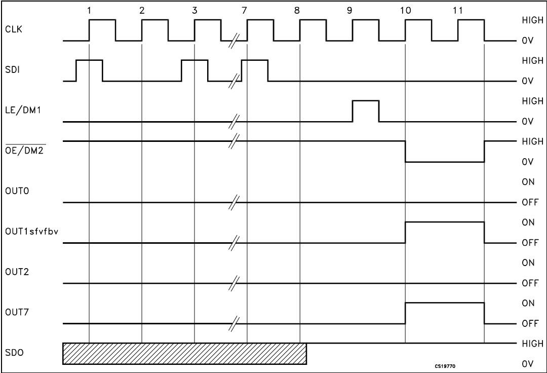
Figure 7. Timing diagram
