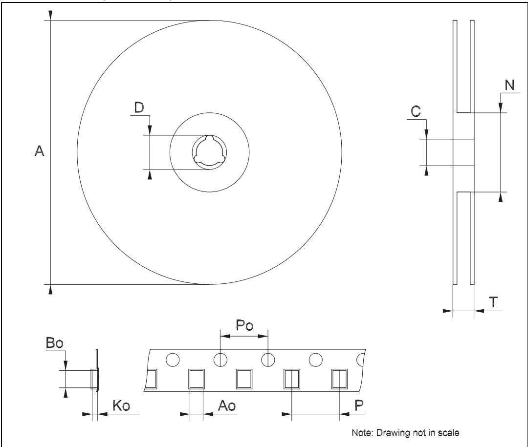
Figure 23. Tape and reel for HTSSOP16 EP and TSSOP16
