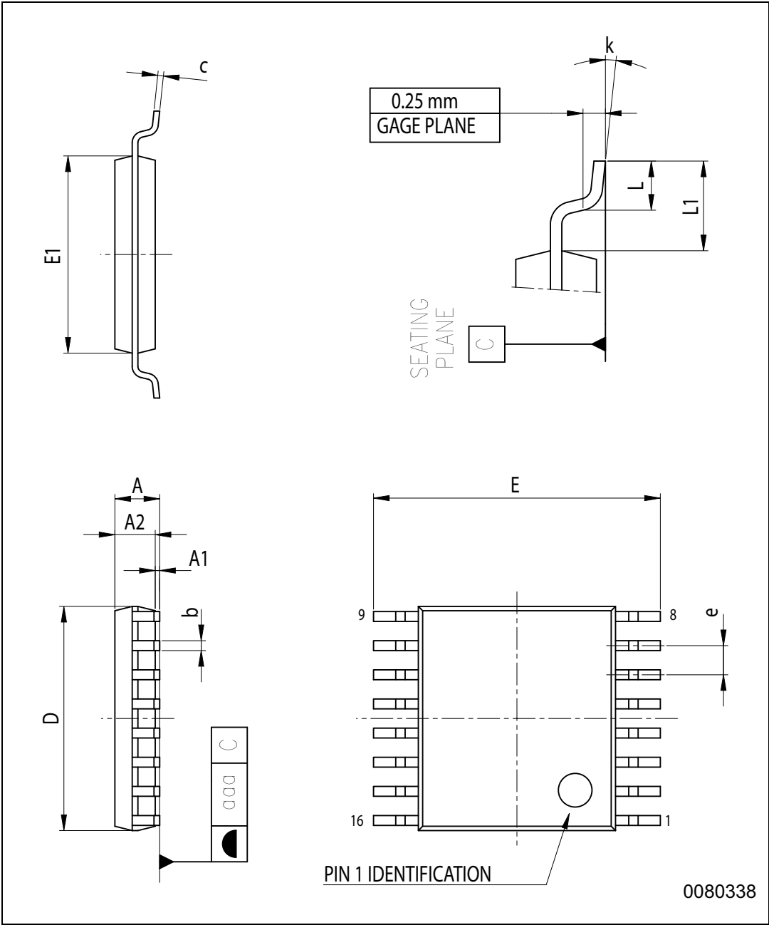
Figure 20. TSSOP16 mechanical drawing
