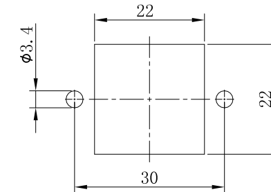
Panel cut out for use without Hoods/housings
