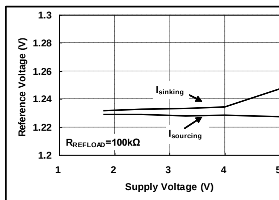
Reference Voltage vs. Supply Voltage
