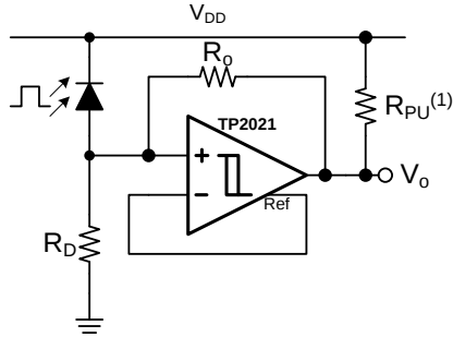
Figure 7. IR Receiver
