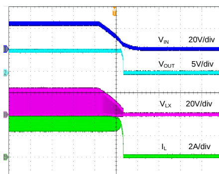
Shutdown from V_{IN} ( V_{IN}=24V , V_{OUT}=5V , I_{OUT}=3A )
