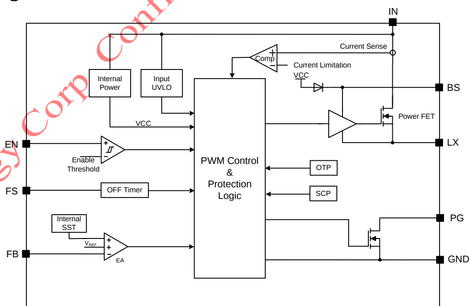
Figure3. Block Diagram
