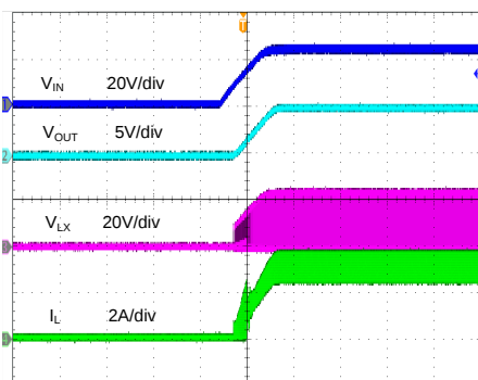
Startup from V_{IN} ( V_{IN}=24V , V_{OUT}=5V , I_{OUT}=3A )
