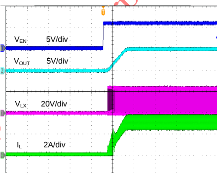
Startup from Enable ( V_{IN}=24V , V_{OUT}=5V , I_{OUT}=3A )
