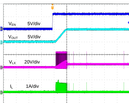
Startup from Enable ( V_{IN}=24V , V_{OUT}=5V , I_{OUT}=0A )
