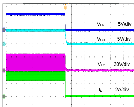
Shutdown from Enable ( V_{IN}=24V , V_{OUT}=5V , I_{OUT}=3A )
