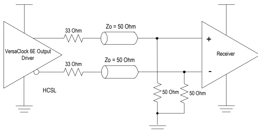
Figure 19. HCSSL Receiver Terminated
