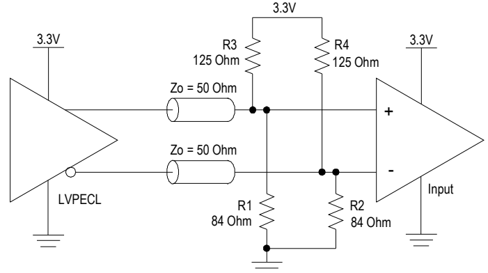
Figure 15. 3.3V LVPECL Output Termination (2)
