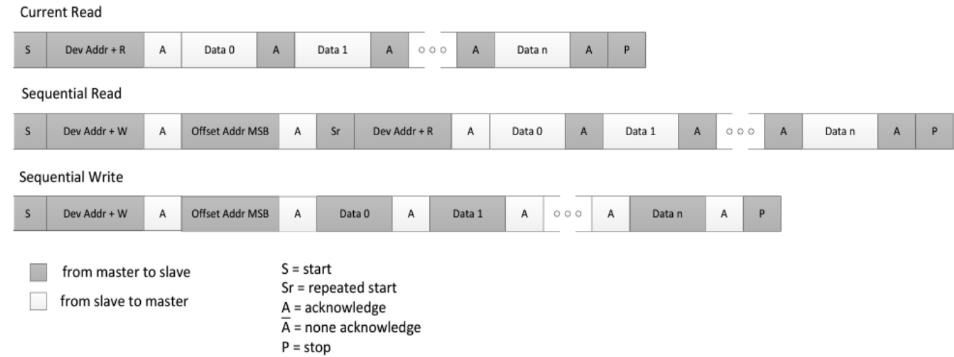
Figure 6: Slave Read and Write Cycle Sequencing
