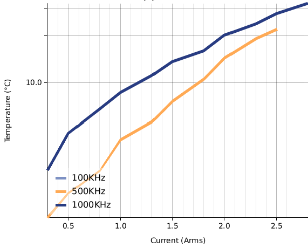
Ripple Current
