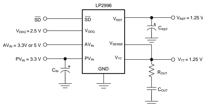
Figure 24. SSTL-2 Implementation with Higher Voltage Rails
