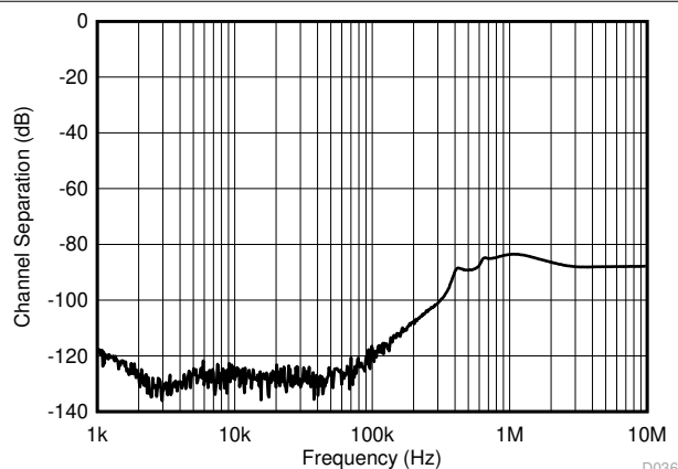
Figure 7-36. Channel Separation
