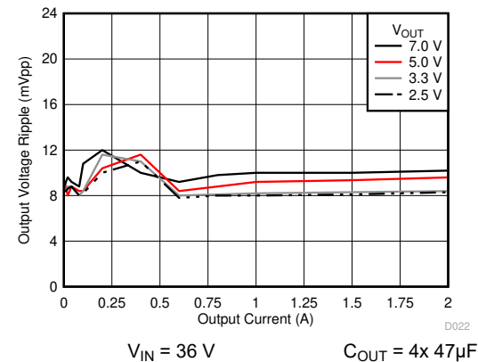
Figure 6-20. Voltage Ripple versus Output Current
