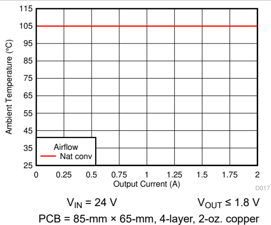
Figure 6-15. Safe Operating Area
