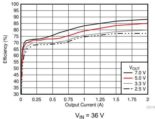
Figure 6-17. Efficiency versus Output Current
