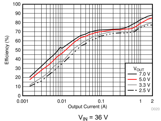
Figure 6-18. Efficiency versus Output Current
