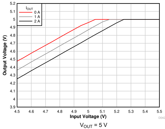
Figure 7-9. Voltage Dropout
