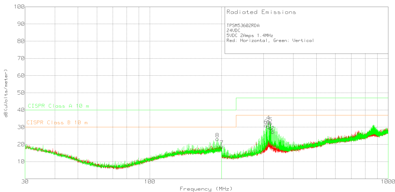
Figure 10-5. Radiated Emissions 24-V Input, 5-V Output, 2-A Load
