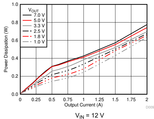
Figure 6-8. Power Dissipation versus Output Current
