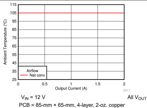
Figure 6-10. Safe Operating Area
