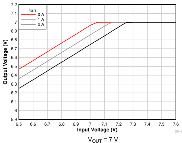
Figure 7-11. Voltage Dropout
