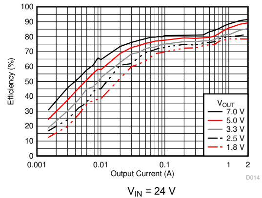
Figure 6-12. Efficiency versus Output Current
