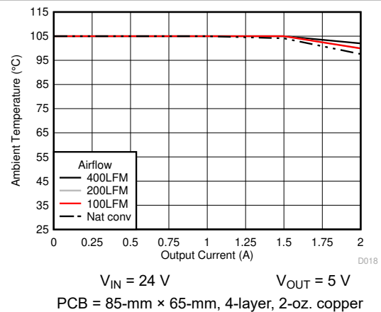
Figure 6-16. Safe Operating Area
