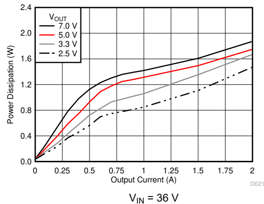
Figure 6-19. Power Dissipation versus Output Current
