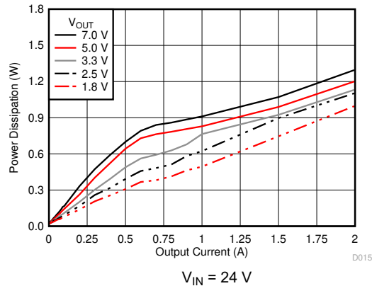
Figure 6-13. Power Dissipation versus Output Current
