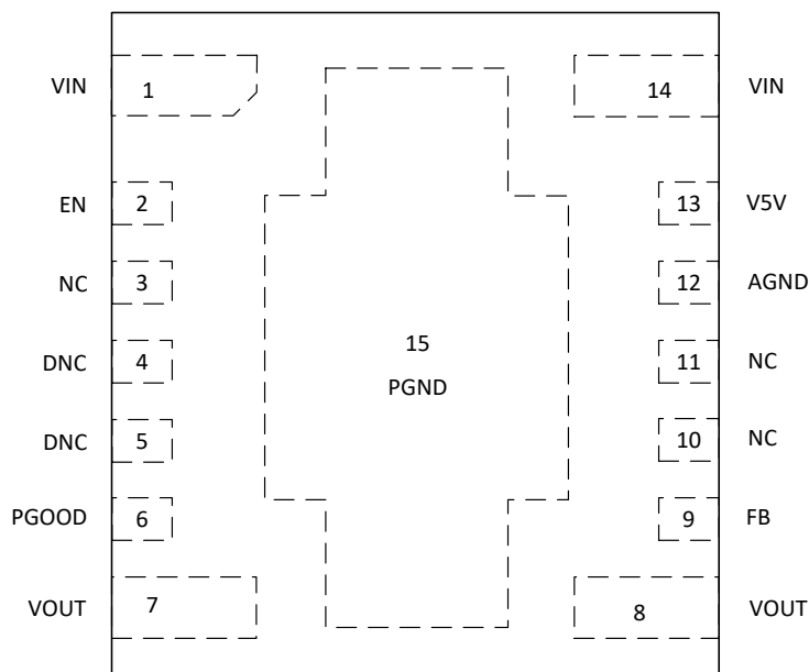
Figure 5-1. RDA Package 15-Pin QFN Top View
