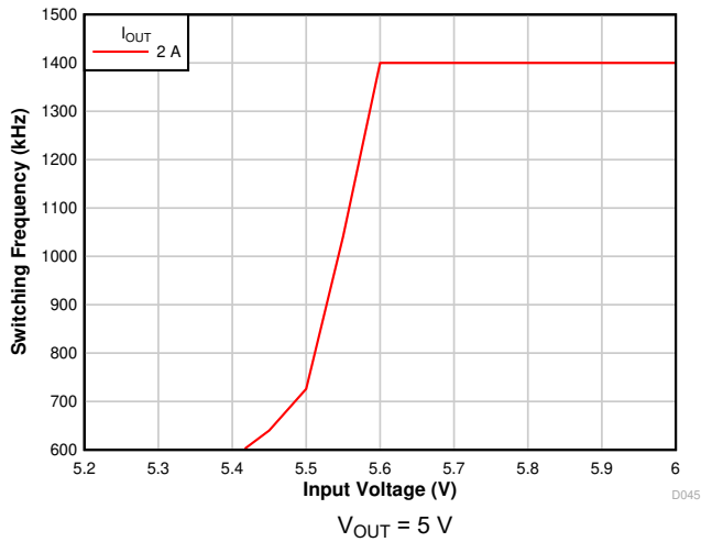
Figure 7-10. Frequency Foldback
