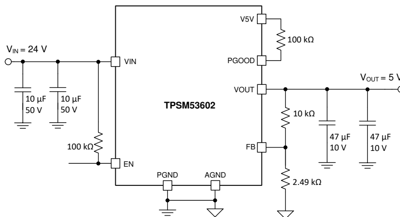
Figure 8-1. TPSM53602 Typical Schematic
