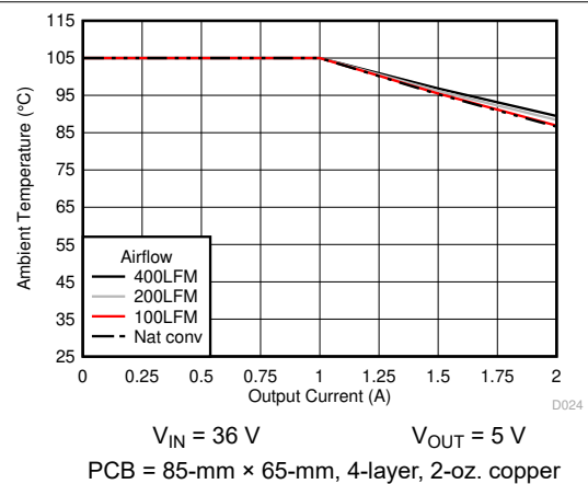
Figure 6-22. Safe Operating Area
