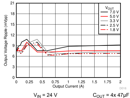
Figure 6-14. Voltage Ripple versus Output Current
