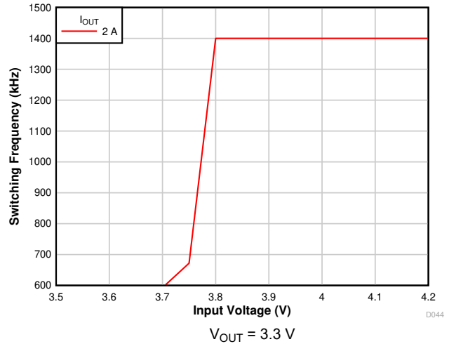
Figure 7-8. Frequency Foldback
