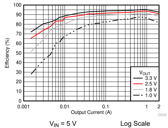
Figure 6-2. Efficiency versus Output Current
