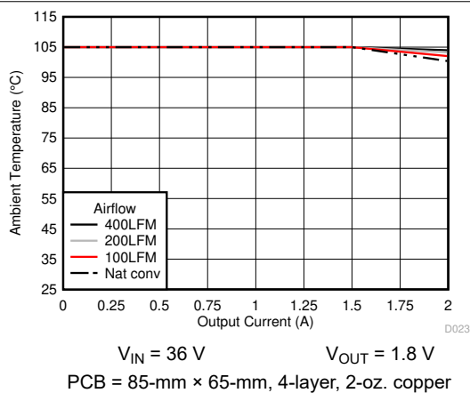
Figure 6-21. Safe Operating Area
