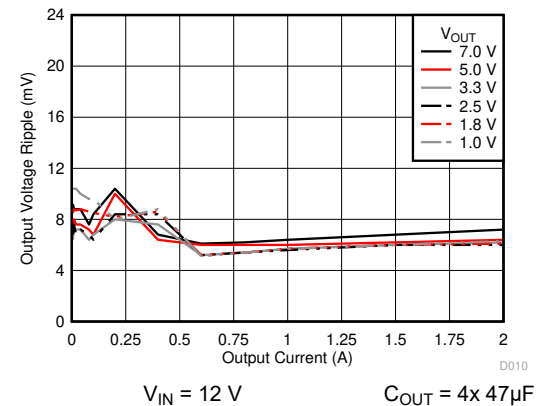
Figure 6-9. Voltage Ripple versus Output Current
