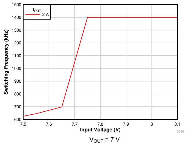
Figure 7-12. Frequency Foldback
