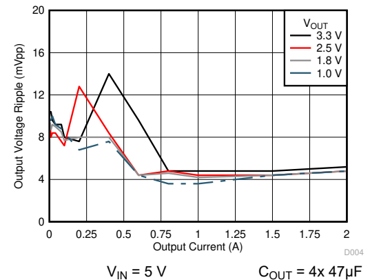
Figure 6-4. Voltage Ripple versus Output Current
