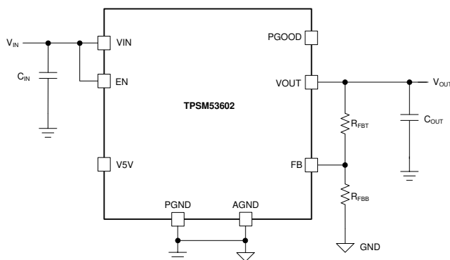
Simplified Schematic
