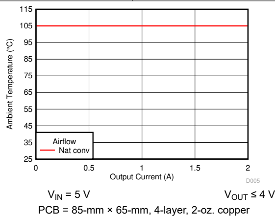
Figure 6-5. Safe Operating Area
