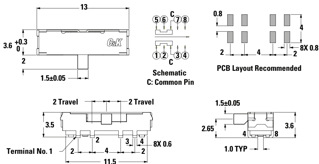
Right Angle Mount SMT - J Bend JS203011JAQN DP3T Shown in position B. Available in tape & reel only
