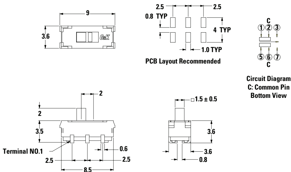
Vertical Mount SMT - J Bend JS202011JCQN DPDT Shown in position B. Available in tap & reel only
