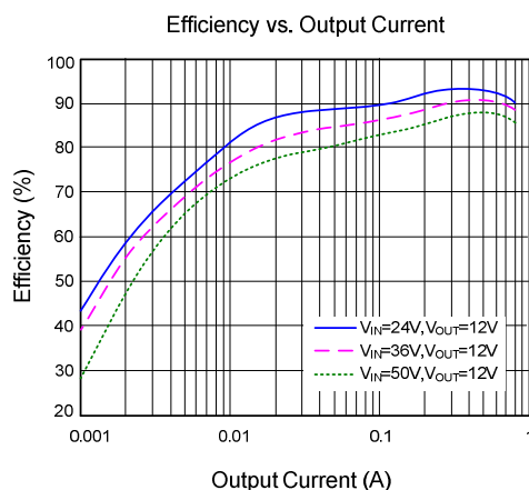
Figure 2. Efficiency
