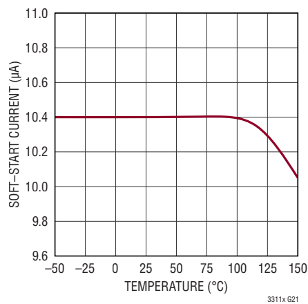
Soft-Start Current
