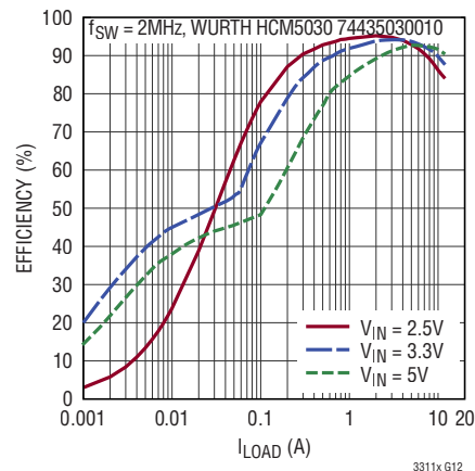
Efficiency, V_{OUT} = 1.8V Pulse-Skipping Mode Operation
