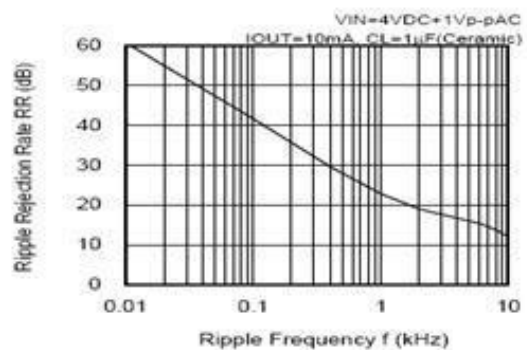
Figure 6: Ripple suppression
