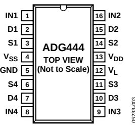
Figure 3. ADG444 (DIP/SOIC)
