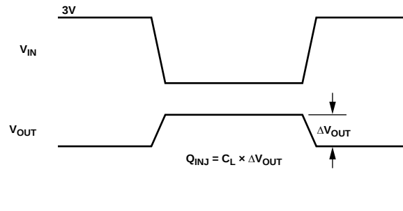
Figure 18. Charge Injection
