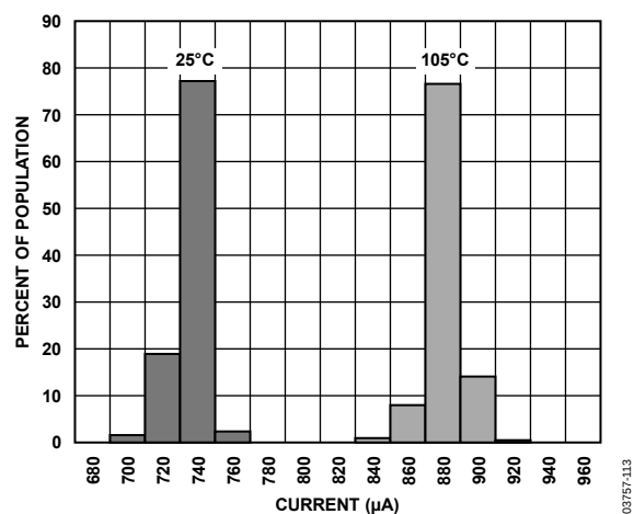
Figure 34. Supply Current vs. Temperature
