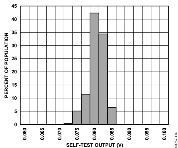
Figure 33. Y-Axis Self Test Response at 25°C
