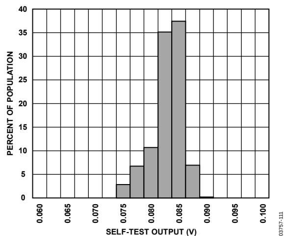
Figure 31. X-Axis Self Test Response at 25°C
