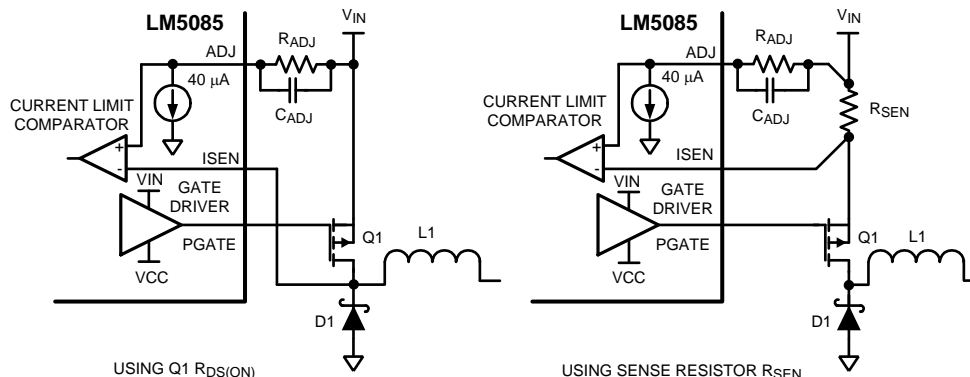
Figure 23. Current Limit Sensing
