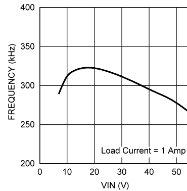
Figure 29. Frequency vs. V_{IN} (Circuit of Figure 24 )
