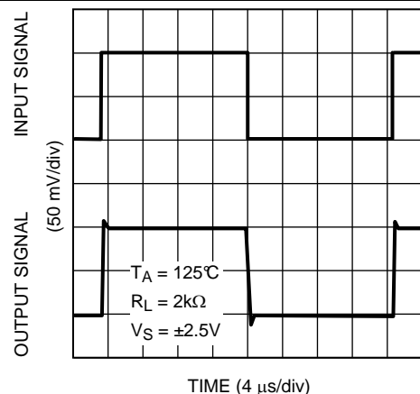
Figure 30. Noninverting Small Signal Pulse Response
