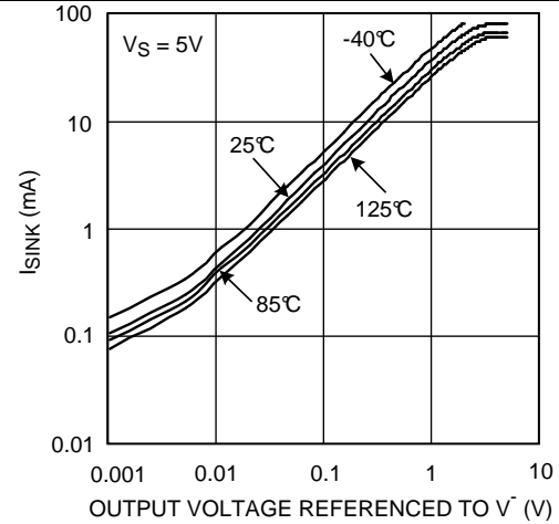
Figure 8. I_{SINK} vs V_{OUT}
