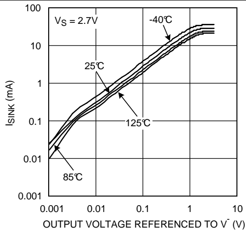
Figure 7. I_{SINK} vs V_{OUT}
