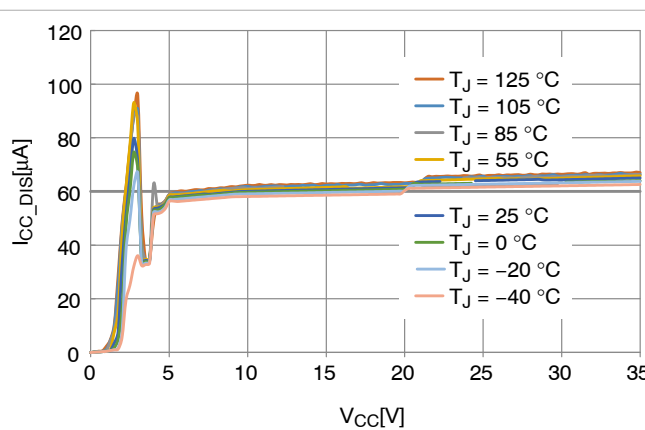
Figure 16. Current Consumption in Disable Mode, V_{CS} = 4 \text{ V}, t > t_{LLD}
